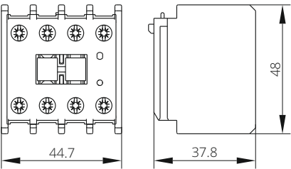
NDL4 Two and four-pole snap-on auxiliary switch blocks (mounting on a basic contactor)
